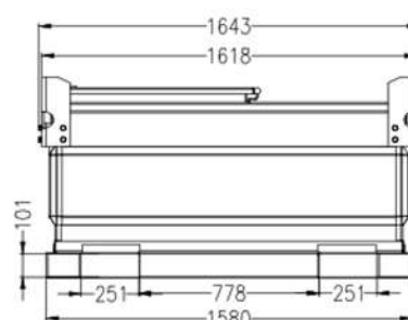
ELEVATION VIEW
