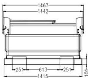
ELEVATION VIEW
