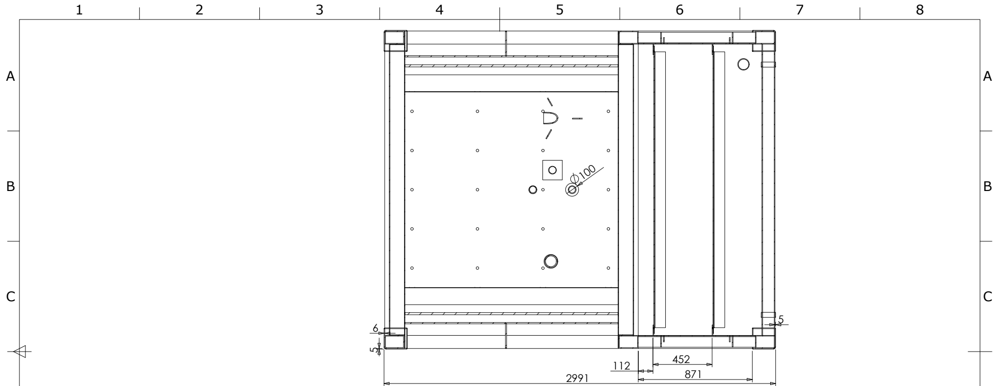
SECTION E-E
